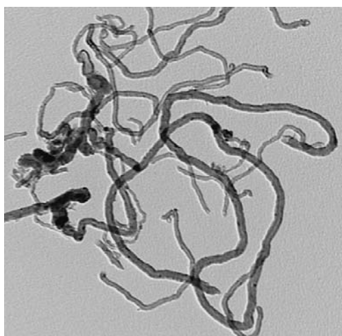
Figure 6.1. Carbon nanotubes
