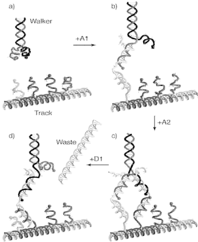
Figure 6.10. Walking molecules
